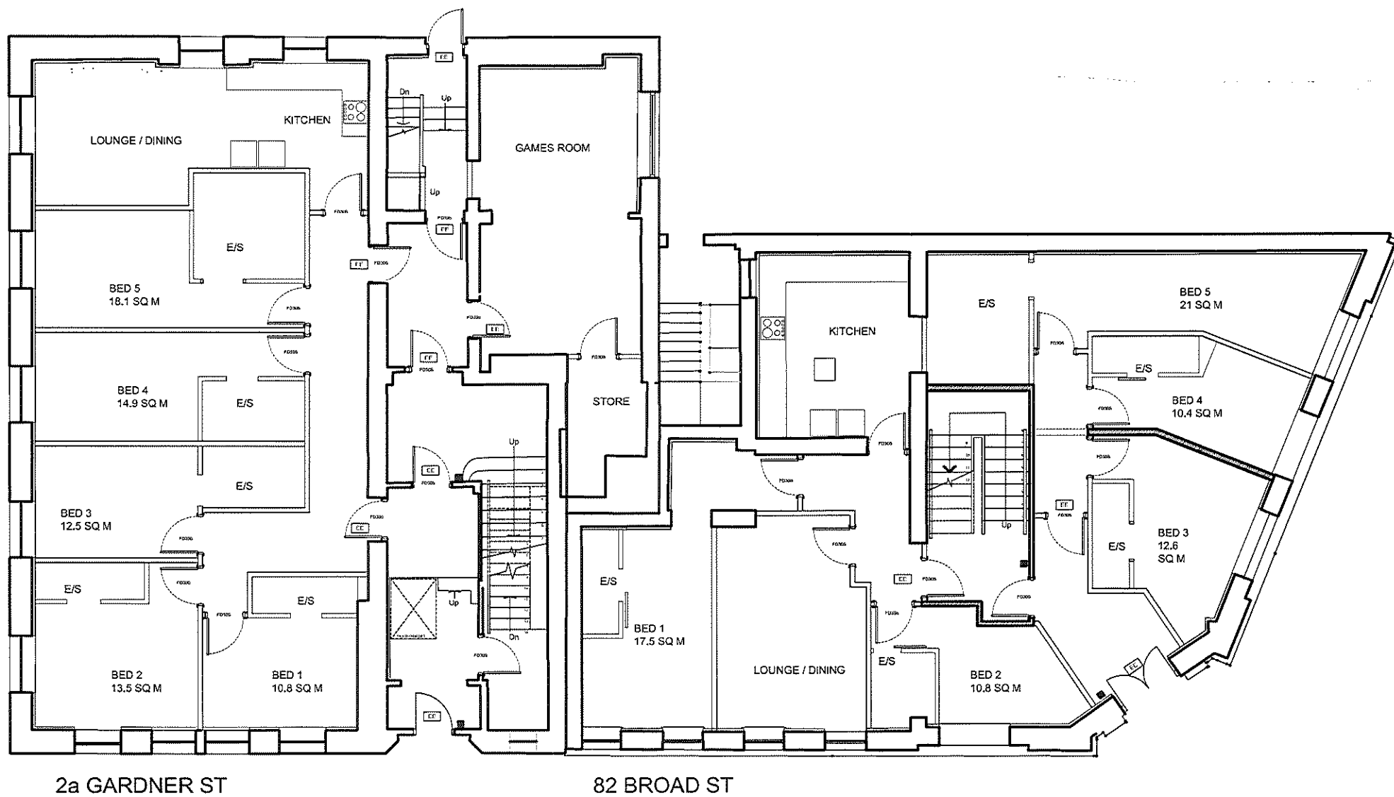
Ground Floor Plan - Areas
