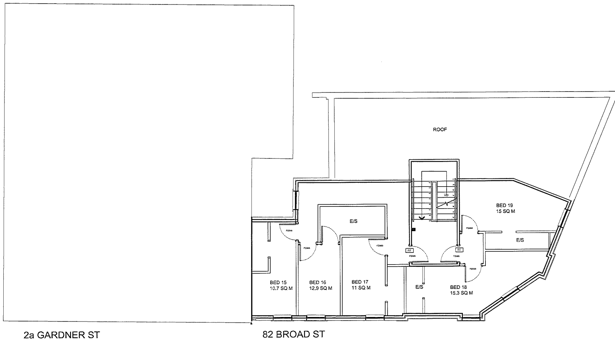
Third Floor Plan - Areas
